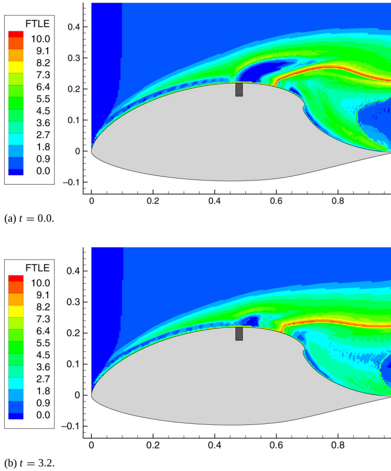
Fig. 13. FTLE field on the airfoil at different times. A moving LCS following the separation profile is clearly visible. For the complete movie see http://www.lekien.com/francois/papers/qLCS . (For interpretation of the references to colour in this figure legend, the reader is referred to the web version of this article.)
