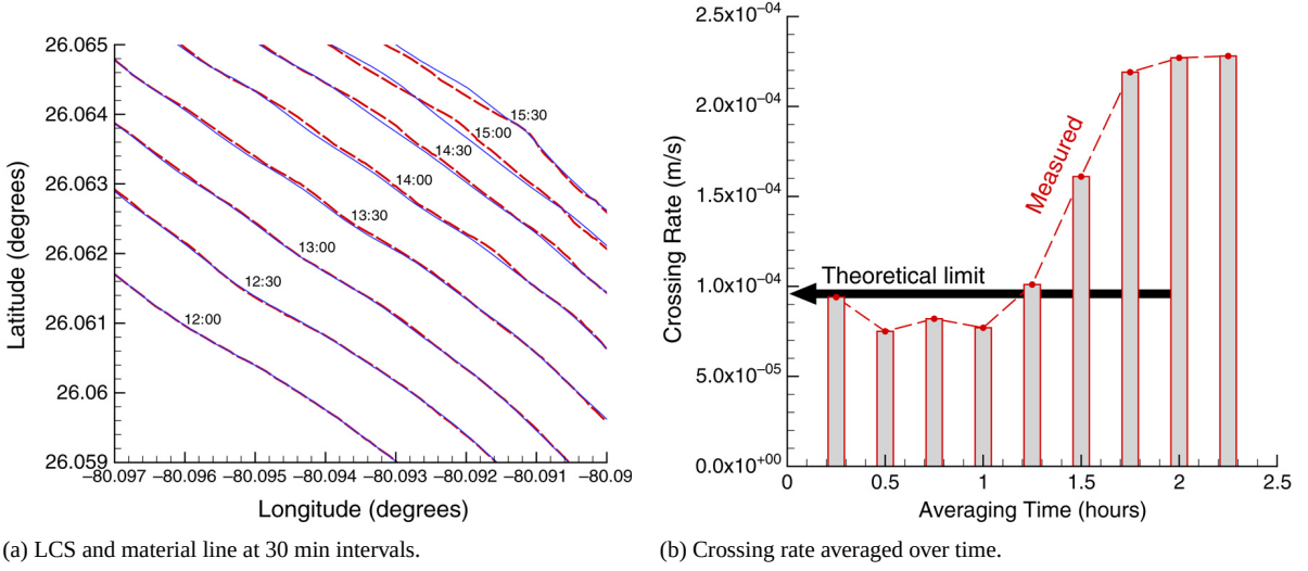
Fig. 12. Panel (a) shows a comparison between the location of the LCS, c_{t+\tau}(s) at different increments of times, \tau , (solid blue curves) with the location of the advected material line, which initially corresponds to c_t(s) (dashed red curves). Panel (b) shows the average crossing rate along the LCS as a function of time; notice that the limiting value for the flux is 10^{-4} m/s. (For interpretation of the references to colour in this figure legend, the reader is referred to the web version of this article.)
